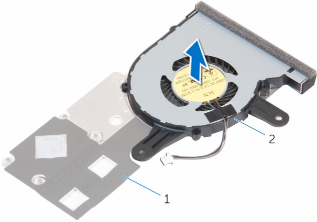
1 heat sink
