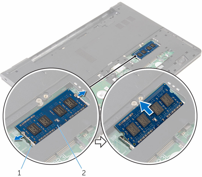
1 securing clips (2)
